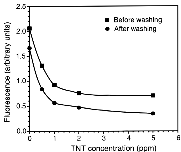
Figure 4. Displacement immunoassays with sol-gel encapsulated Ab showing the effect of washing excess TNT-FITC prior to displacement. [\text{Ab}] = 2.7 \mu\text{M} , initial [\text{TNT-FITC}] = 20 \text{ ppm} .
