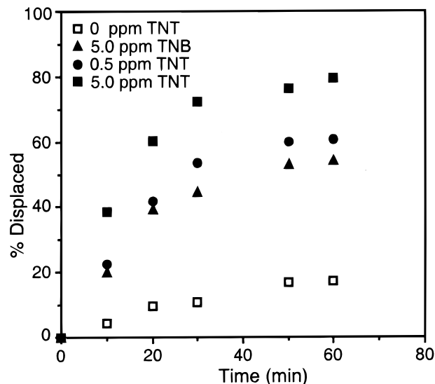
Figure 5. Displacement of TNT-FITC by unlabeled TNT or TNB in aged silica gels. The slight loss in signal in the 0 ppm TNT sample is likely due to incomplete washing of excess TNT-FITC before displacement.
