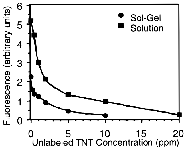
Figure 1. Competitive immunoassay results for sol-gel encapsulated Ab and surface immobilized Ab. In the sol-gel experiment, [Ab] = 1.35 \mu\text{M} and [TNT-FITC] = 0.5 \text{ ppm} . In the solution experiment, Ab was adsorbed on the surface of polystyrene with [TNT-FITC] = 5.0 \text{ ppm} .
